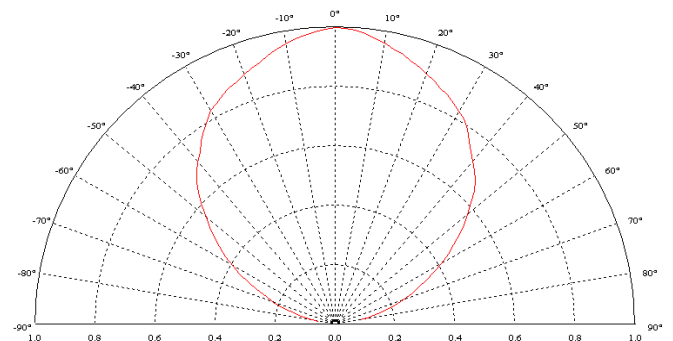
Radiation Pattern
