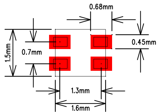
PCB Solder Pad Design
