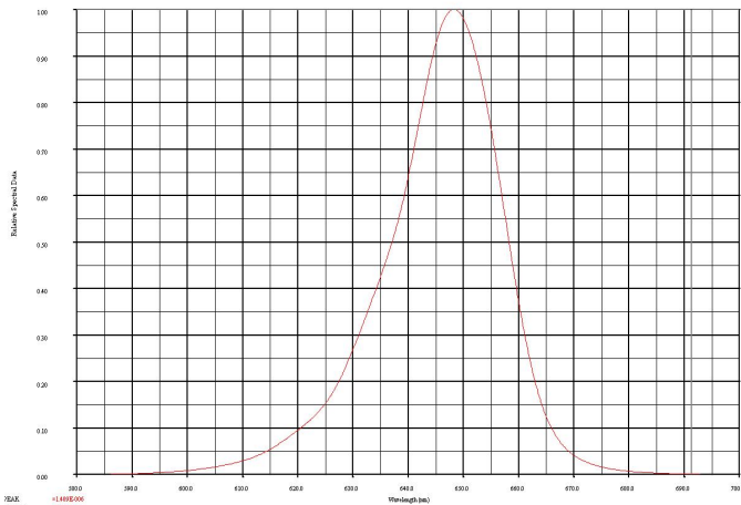
Spectral Output
