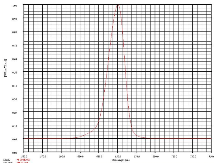
Spectral Output
