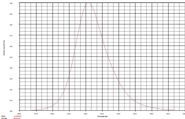
Spectral Output
