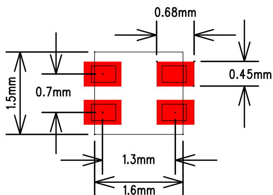
PCB Solder Pad Design
