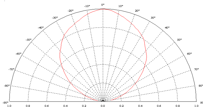
Radiation Pattern
