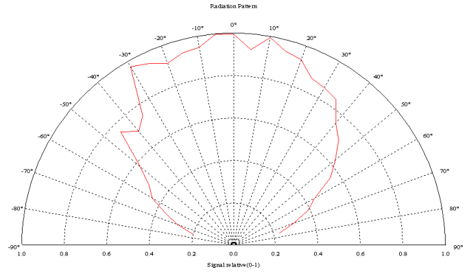
Radiation Pattern
