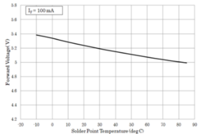
■ Solder Point Temperature vs Forward Voltage
