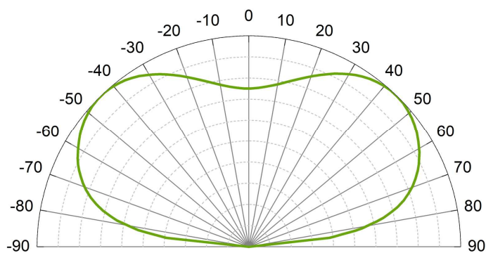
Radiation pattern
