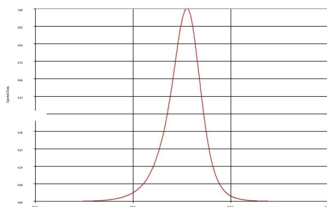
570nm Spectral Response
