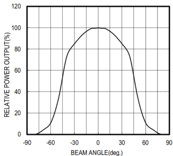
RADIATION PATTERN
