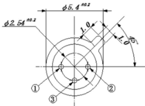
① Case ② Cathode ③ Anode Dimensions (Unit:mm)
