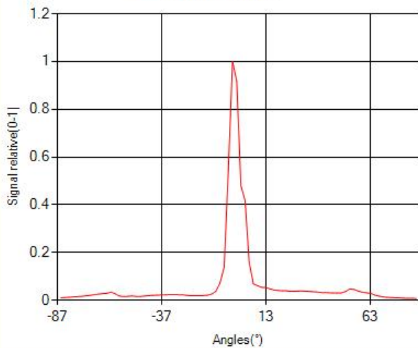
RADIATION DISTRIBUTION
