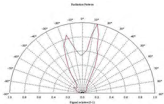
VIEW ANGLE
