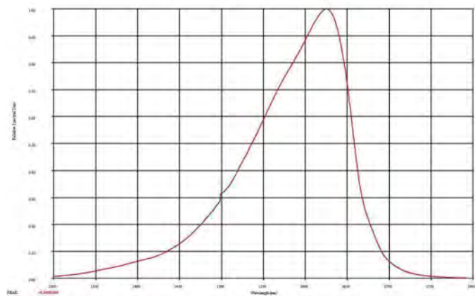
SPECTRAL RESPONSE
