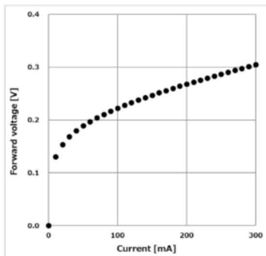
Forward voltage vs. current(typical data)
