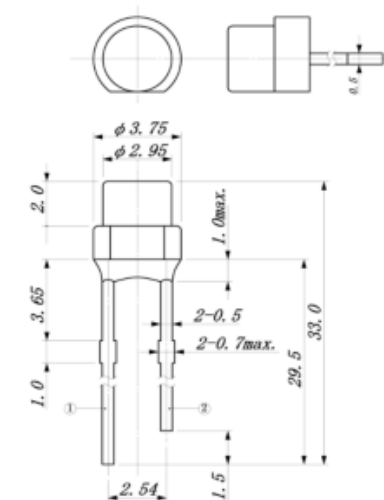
① Anode ② Cathode Dimensions (Unit:mm)
