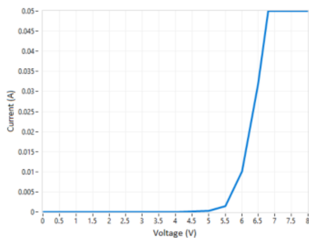
Figure 4. Forward current vs forward voltage T_s = 25^\circ\text{C}
