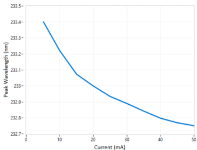
Figure 3. Peak wavelength vs forward current T_s = 25^\circ\text{C}
