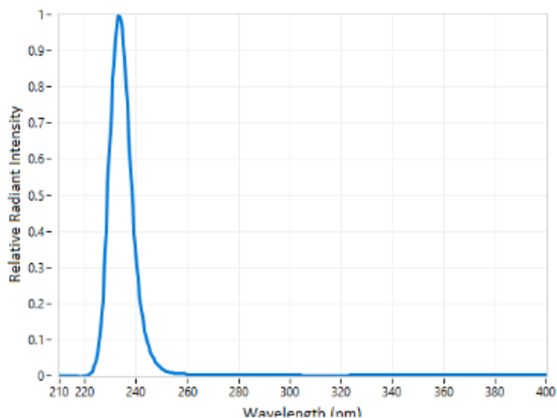
Figure 1. Relative emission intensity vs wavelength T_s = 25^\circ\text{C} , I_f = 20\text{ mA}
