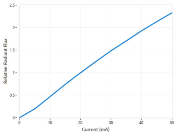
Figure 2. Relative radiant flux vs forward current T_s = 25^\circ\text{C}
