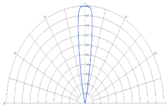
Figure 8. Radiation pattern T_A = 25^\circ\text{C} , I_f = 20 \text{ mA}
