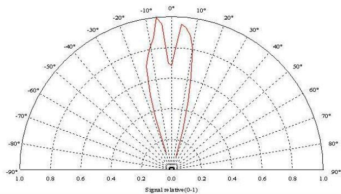
Radiation Pattern
