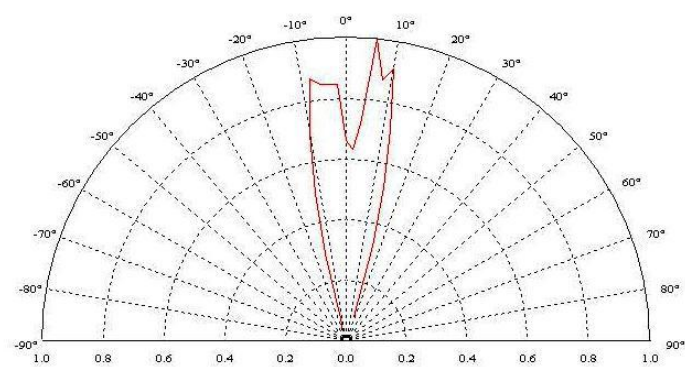
Radiation Pattern
