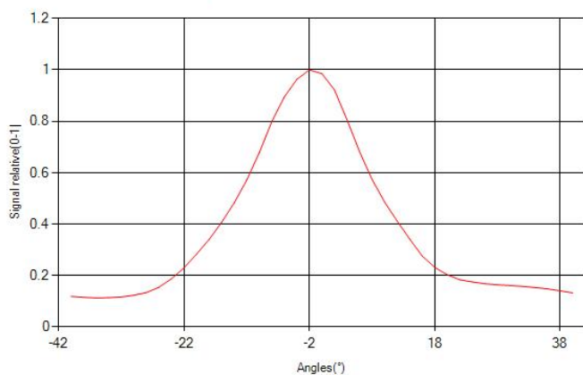
RADIATION DISTRIBUTION
