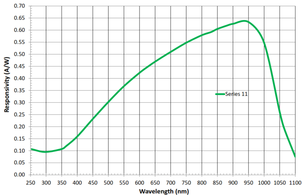
Marktech Optoelectronics Series 11 Responsivity
